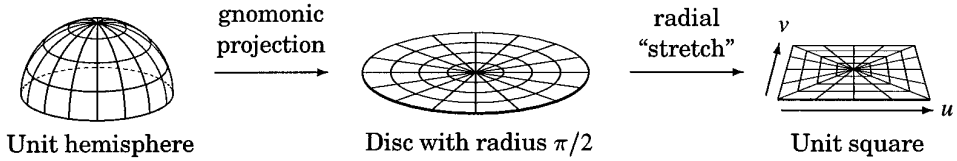
Fig. 2. Angular projection: gnomonic projection and radial “stretch.”
