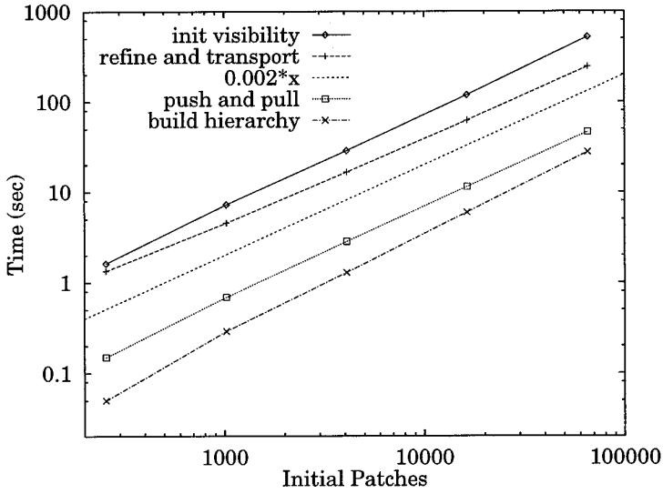
Fig. 4. Time spent in various stages of the new method as a function of the number of initial patches.
