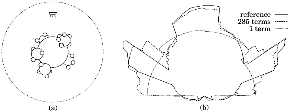
Fig. 6. Glossy sphereflake: (a) sketch of the geometry; (b) polar plots of cluster approximations.
