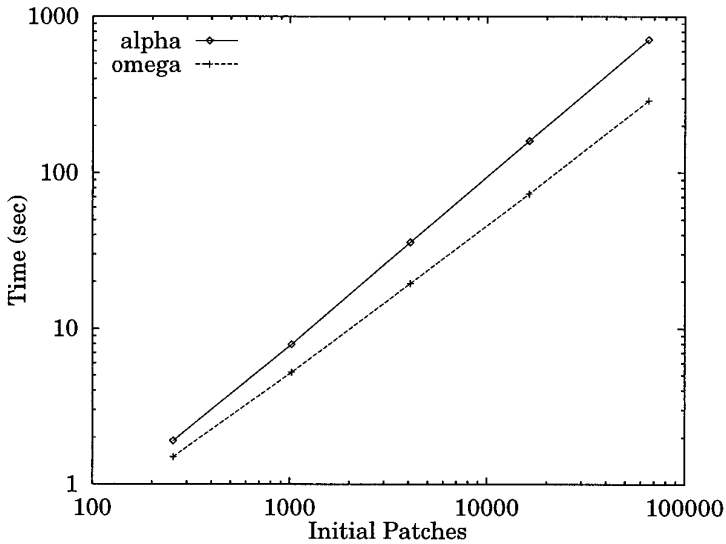
Fig. 5. Time spent by different clustering algorithms as a function of the number of initial patches.
