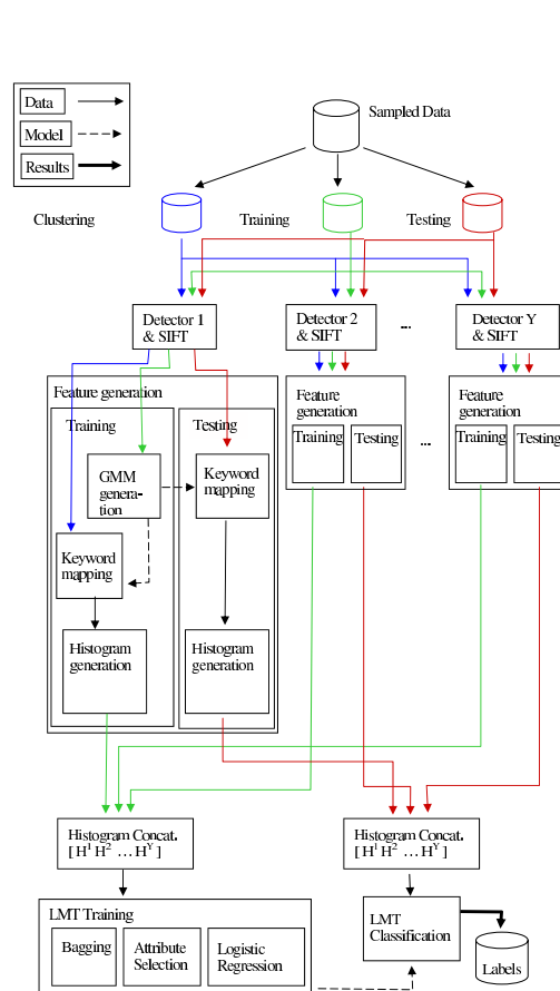
Fig. 5 Object recognition system overview: Feature generation and classification components
