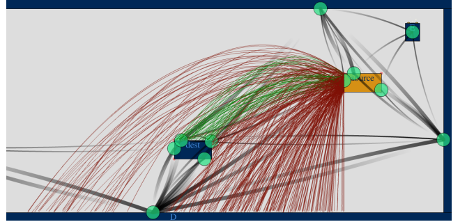
Figure 3: A dense resampling for a clustered edge chosen by the user. The red and green lines show the path of the frog as a result of each sampled action. The green lines are those that hit the target surface and the red lines are those that did not. The platforms are blue with labels to make them distinguishable when the user is determining the degrees of freedom. When a platform is designated as movable, it turns yellow.
