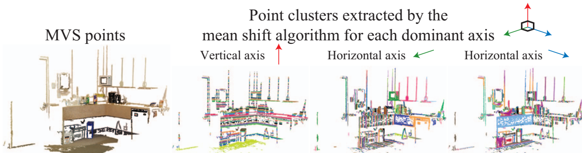
Figure 5. Oriented points reconstructed by [11], and point clusters that are extracted by mean shift algorithm are shown for each of the three dominant directions. Points that belong to the same cluster, and hence, contribute to the same plane hypothesis are shown with the same color.
