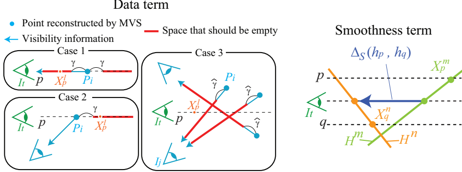
Figure 3. Data term measures visibility conflicts between a plane hypothesis at a pixel and all the reconstructed points \{P_i\} . There are three different cases in which the visibility conflict occurs. The smoothness term in this figure measures the penalty of assigning a hypothesis H^n to pixel q , and a hypothesis H^m to pixel p . See the text for details.
